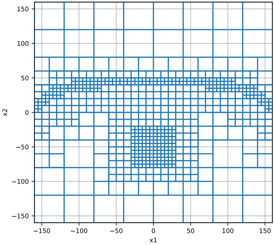
QuadTree Mesh
