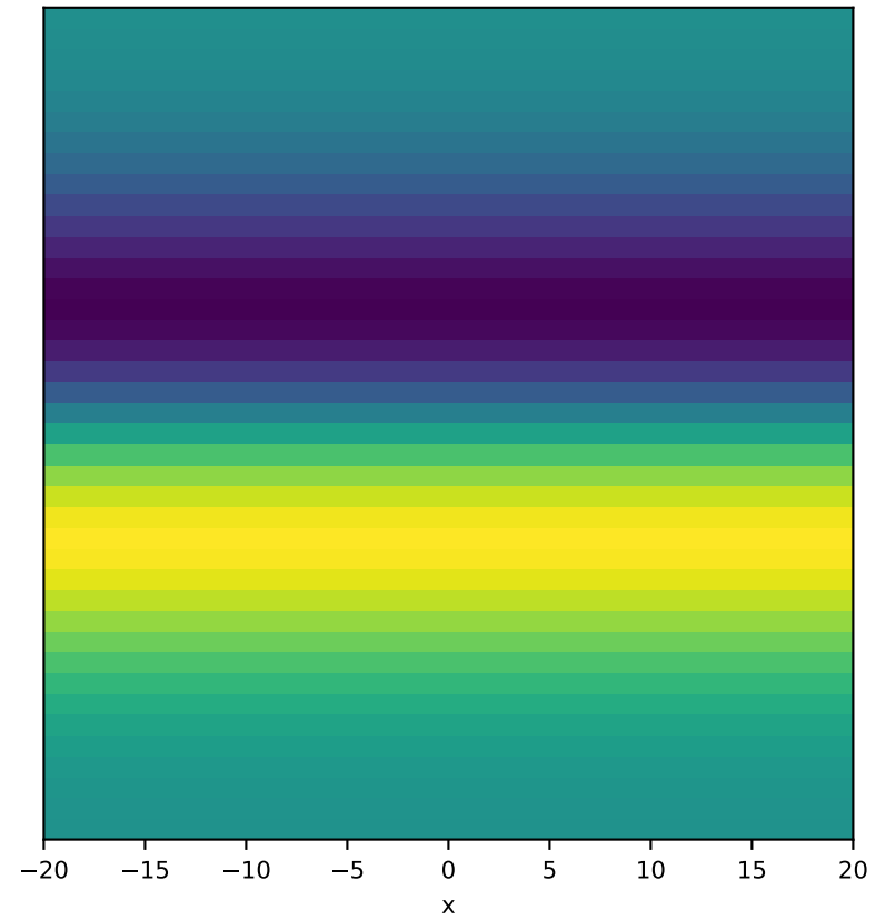
Y-derivative at cell center
