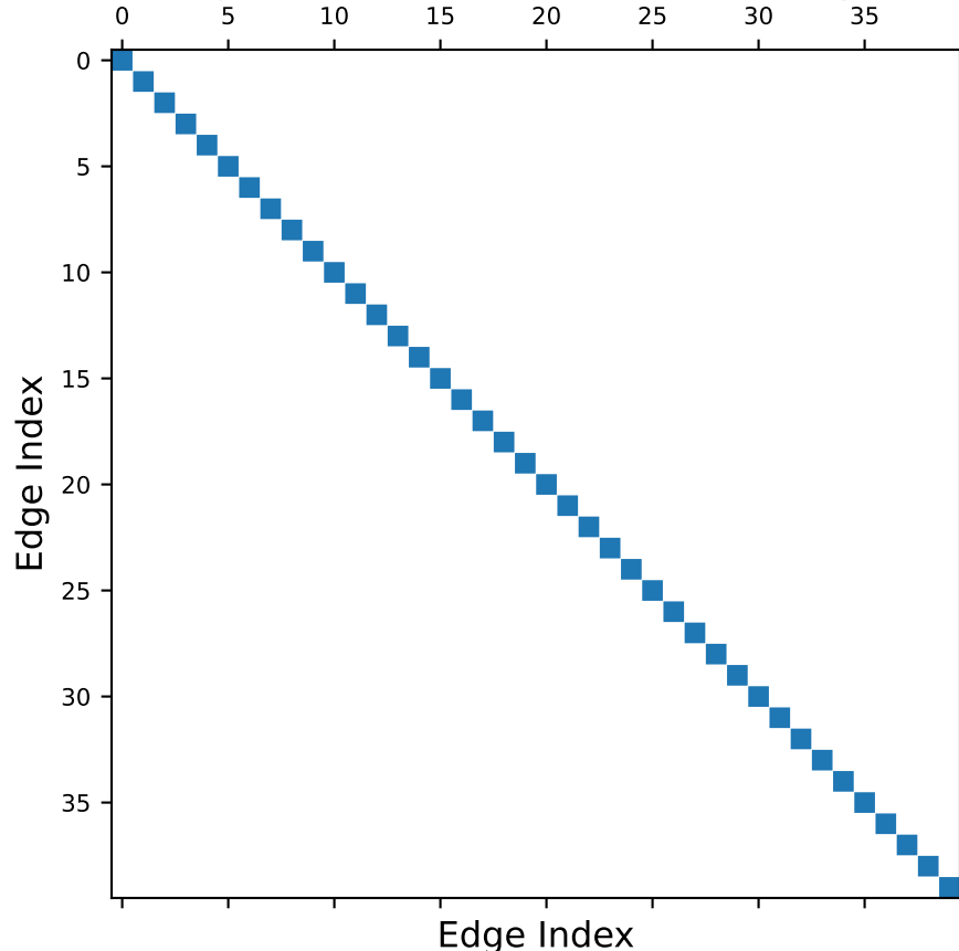
Edge Inner Product Matrix (Isotropic)
