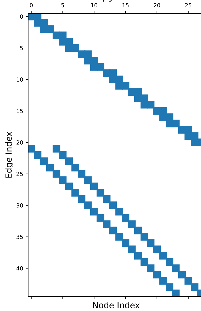
Spy Plot
