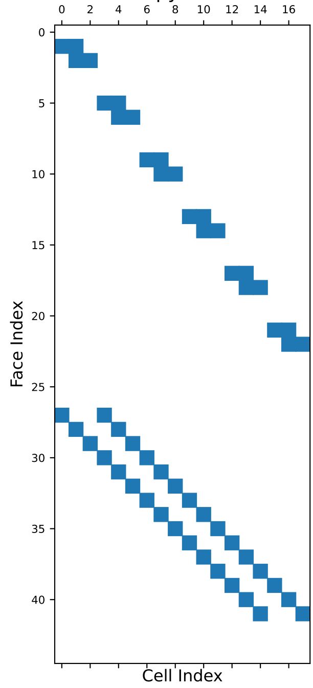
Spy Plot
