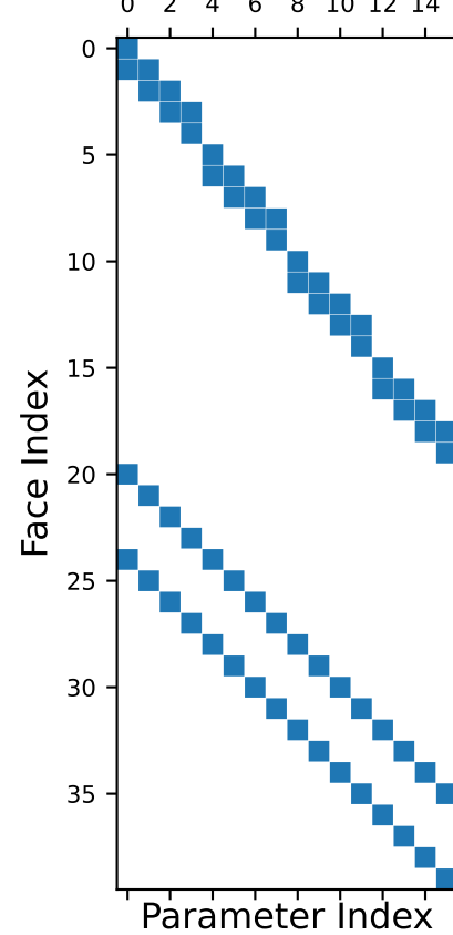
u^T \frac{\partial M(m)}{\partial m} (Isotropic)
