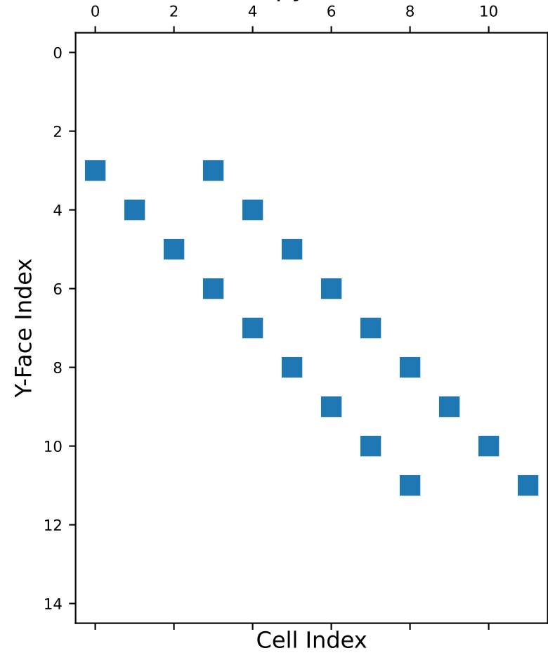
Spy Plot
