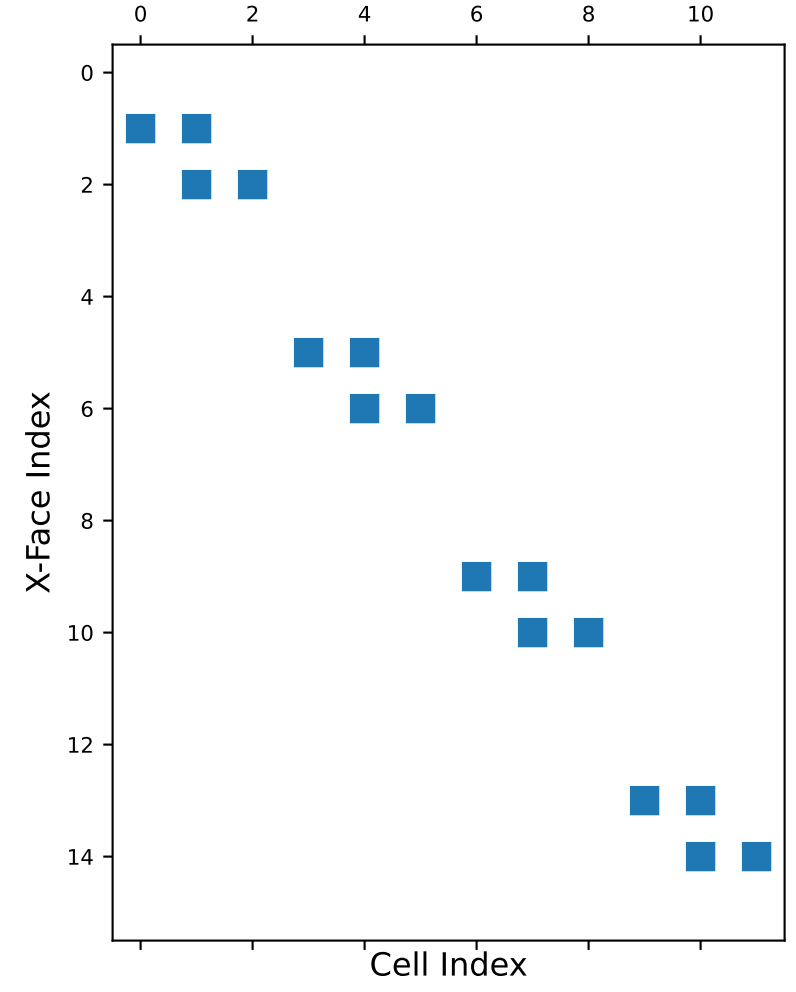
Spy Plot
