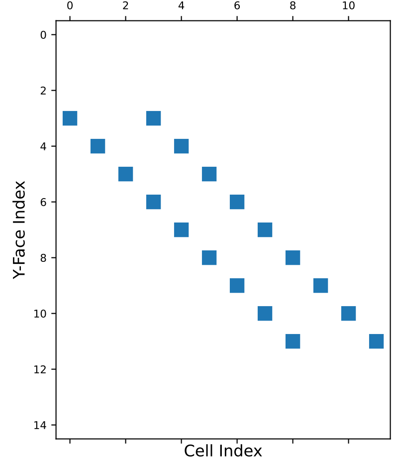
Spy Plot
