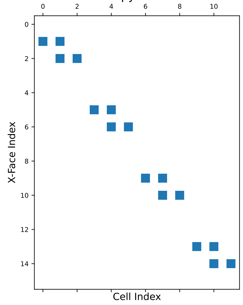
Spy Plot
