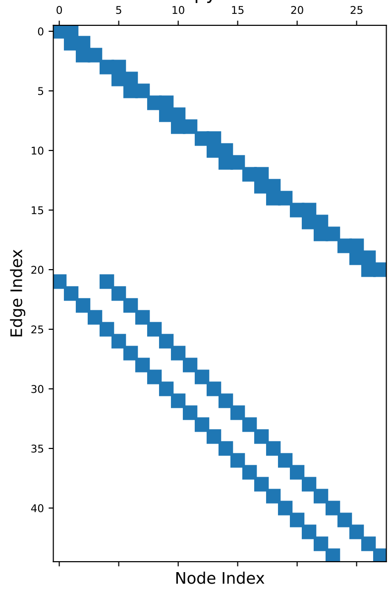
Spy Plot
