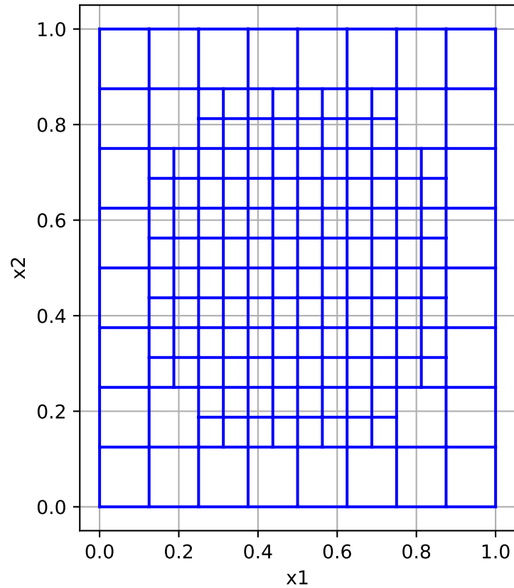
TreeMesh
