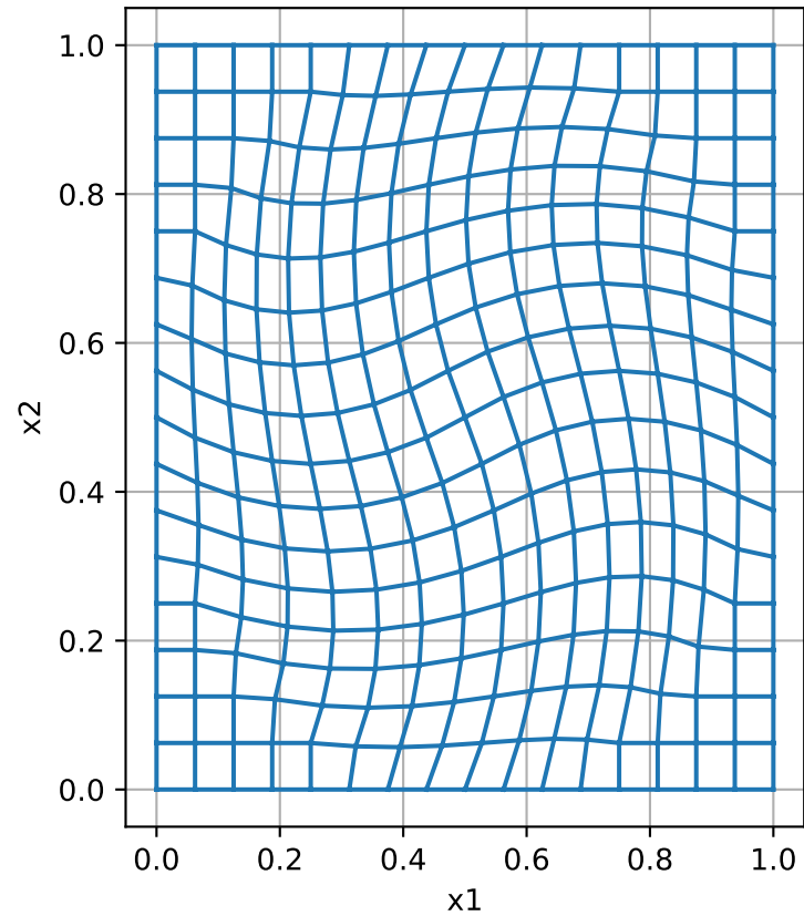
CurvilinearMesh
